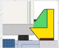
Wiper Seal for Trucks Equipped With Step or Tailgate
